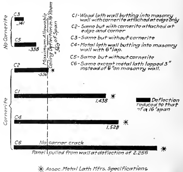
Showing that cornerite prevents corner cracks between partitions and masonry walls even after maximum allowable deflection is reached in joists.
